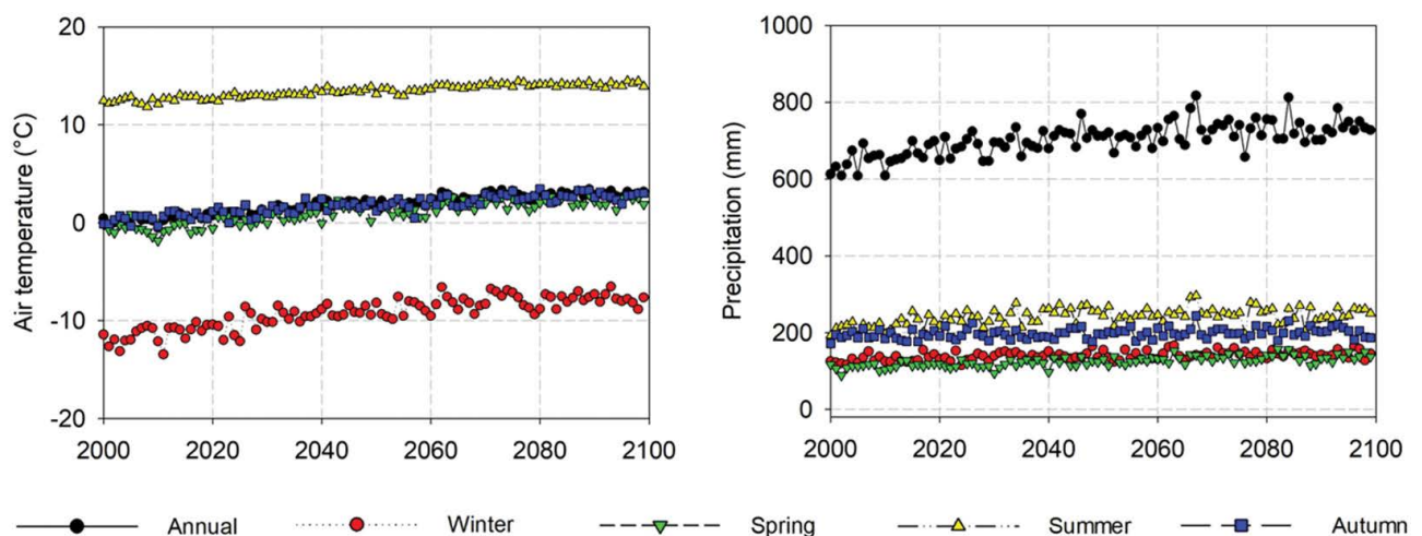
Figure 1. Example Climate Change Scenario Data for Aitik Mine (RCP4.5, 50 km gridded). The data shown are derived by averaging monthly climate data outputs from nine GCMs.
