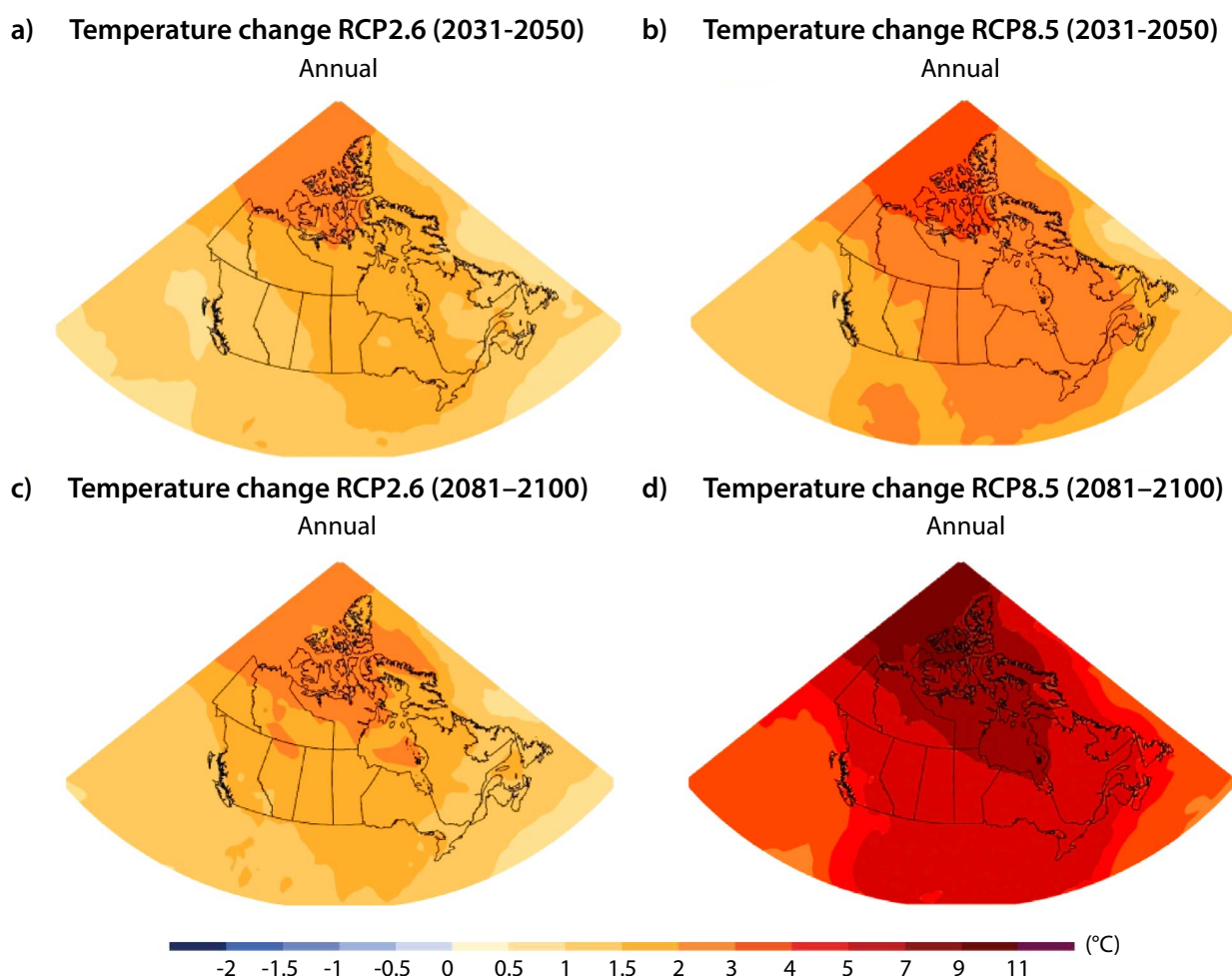
Figure 4: Annual temperature change under a low emission (RCP2.6) and high emission (RCP8.5) scenarios, for the mid-century (2031 to 2050) and end of century (2081 to 2100) time horizons (Reference: Figure 4.8 (fragment) from Bush, E. and Lemmen, D.S., editors (2019): Canada's Changing Climate Report ; Government of Canada, Ottawa, ON. 444 p.).
